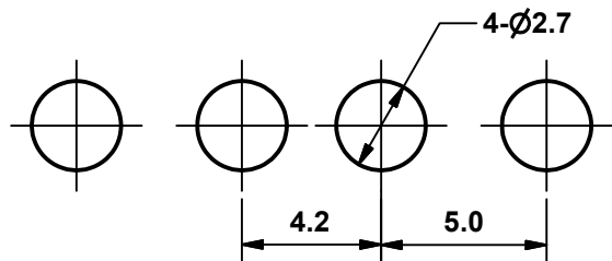
MOUNTING HOLES
